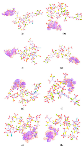
Figure 2: Electrophilic Fukui functions f(r) for (a) Mirabamide A; (b) Mirabamide B; (c) Mirabamide C; (d) Mirabamide D; (e) Mirabamide E; (f) Mirabamide F; (g) Mirabamide G and (h) Mirabamide H—This graphic has been plotted following the Chem-Craft style where the following colors have been assigned to the atoms: C: lilac, H: red, N: yellow, O: green and Cl: blue, and orange and purple are assigned to positive and negative surfaces, respectively.
