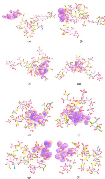
Figure 3: Nucleophilic Fukui functions f^+(r) for (a) Mirabamide A; (b) Mirabamide B; (c) Mirabamide C; (d) Mirabamide D; (e) Mirabamide E; (f) Mirabamide F; (g) Mirabamide G and (h) Mirabamide H—This graphic has been plotted following the Chem-Craft style where the following colors have been assigned to the atoms: C: lilac, H: red, N: yellow, O: green and Cl: blue, and orange and purple are assigned to positive and negative surfaces, respectively.
